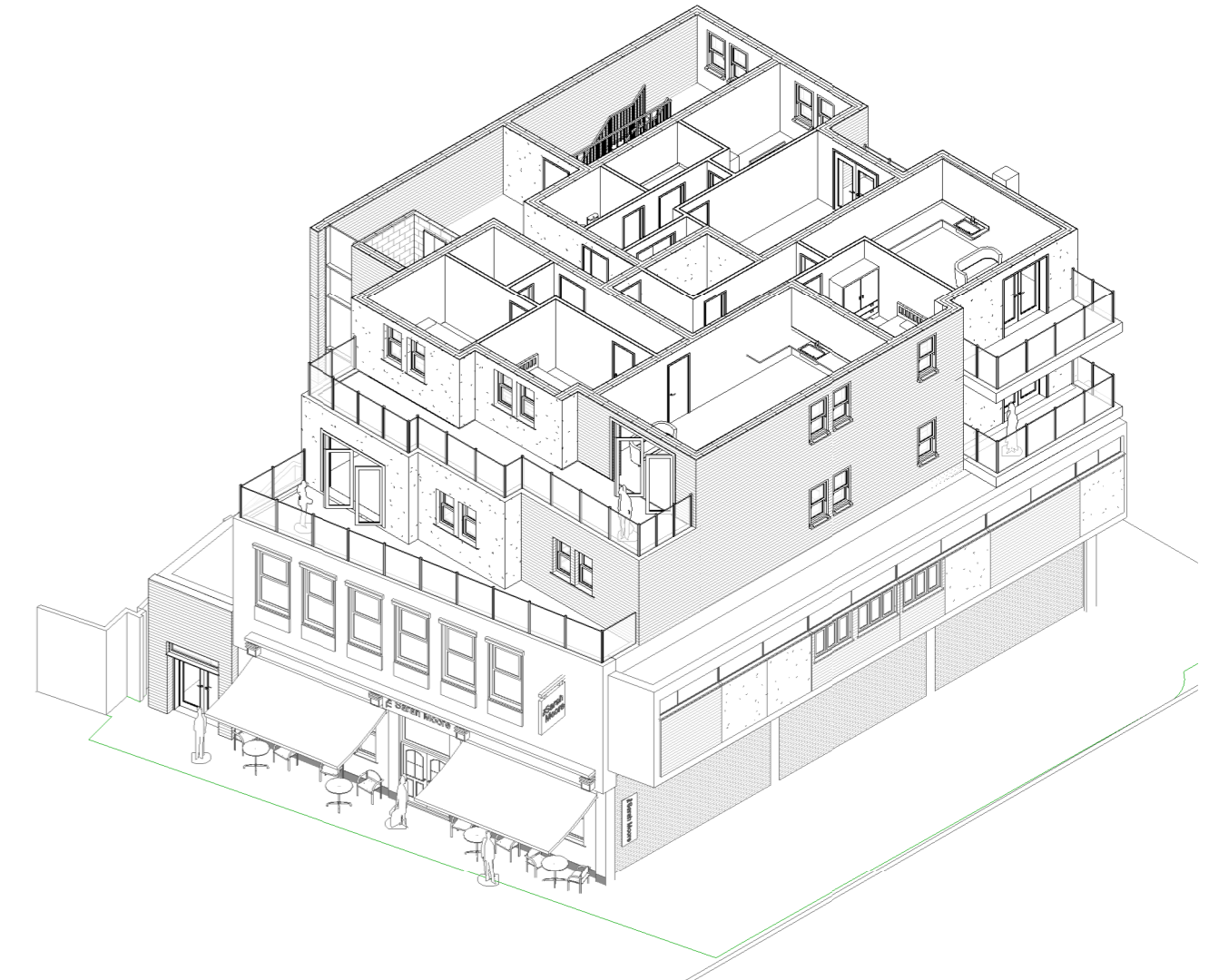
3 Third Floor ISO 3D
